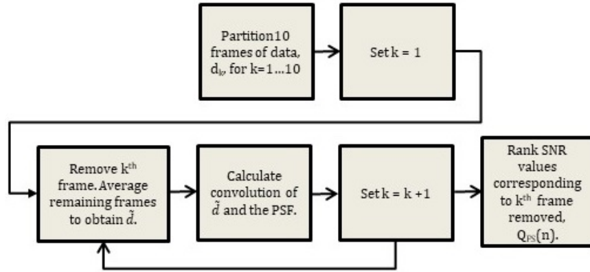
Figure 37. Flow chart of initial processing completed in the short exposure frame selection algorithm.
