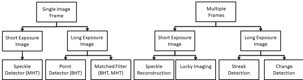
Figure 6. Generalized space object detection techniques depending on number of frames captured and integration times.
